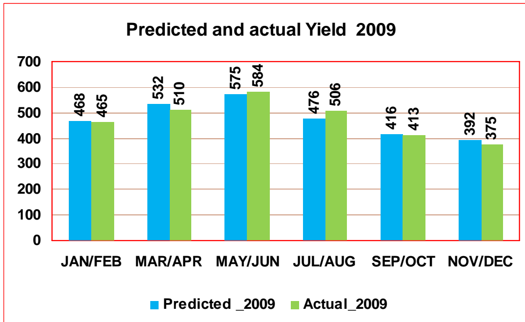
Figure 1: The comparison of actual and forecasted ANCP of 2009
